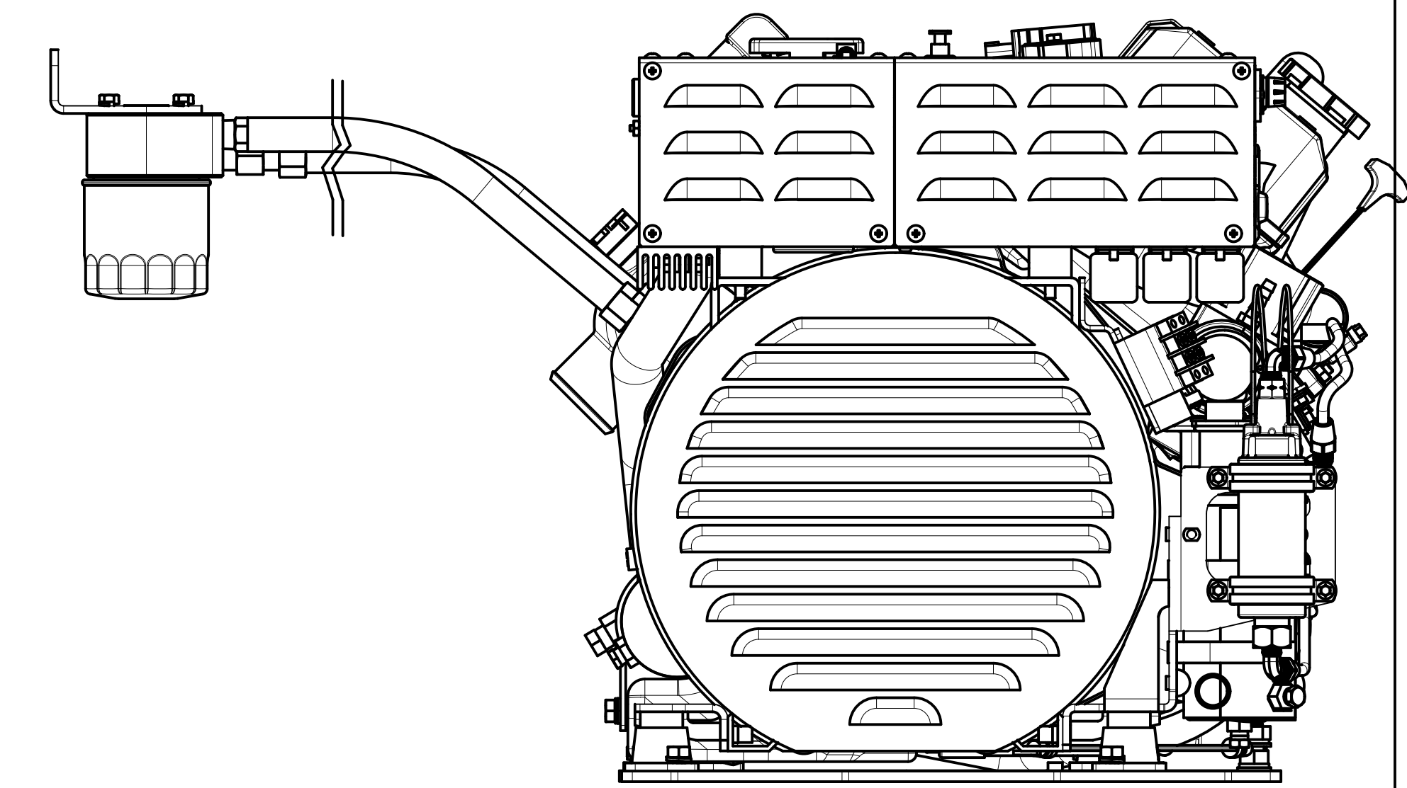
GENERATOR END
