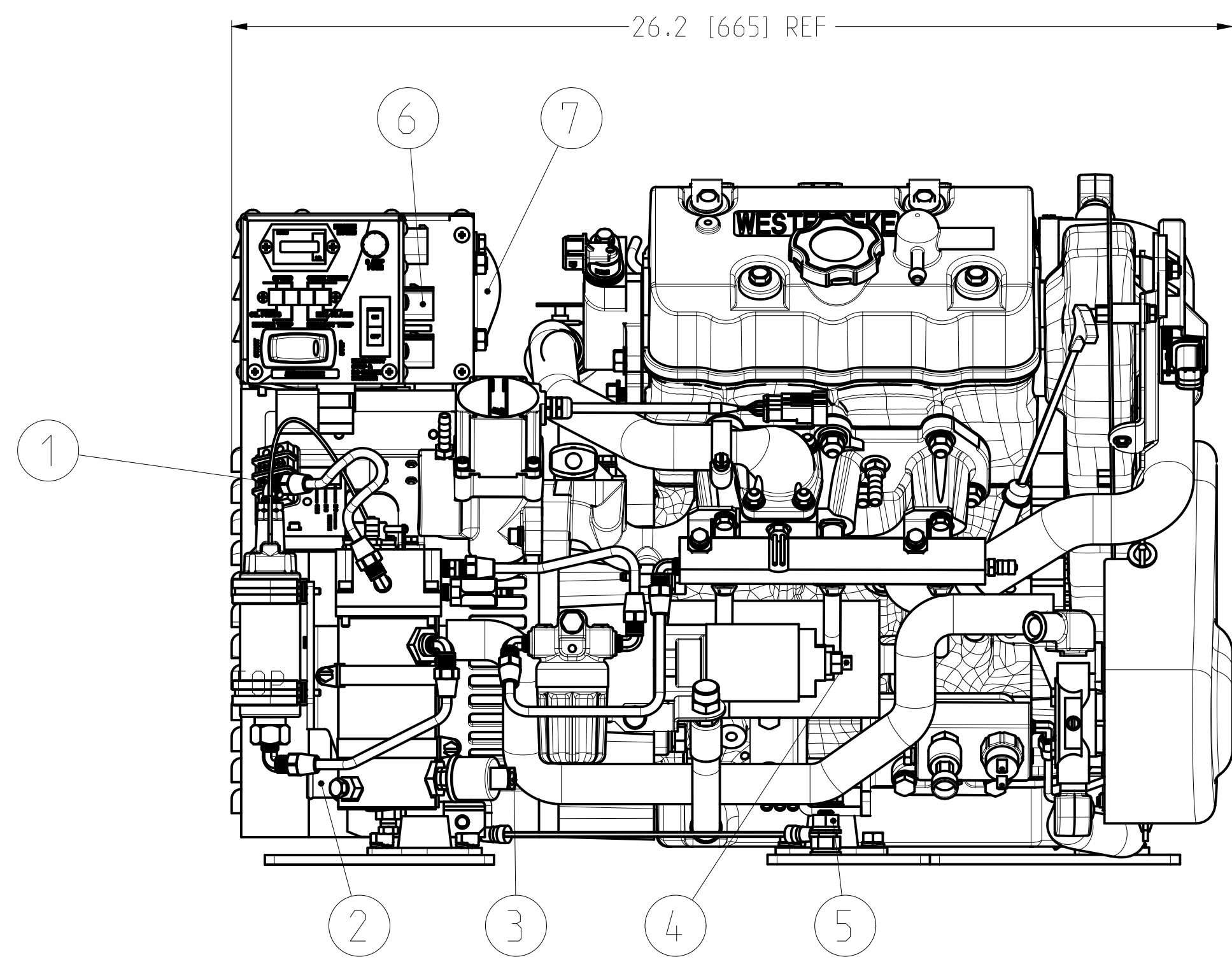
SERVICE SIDE
