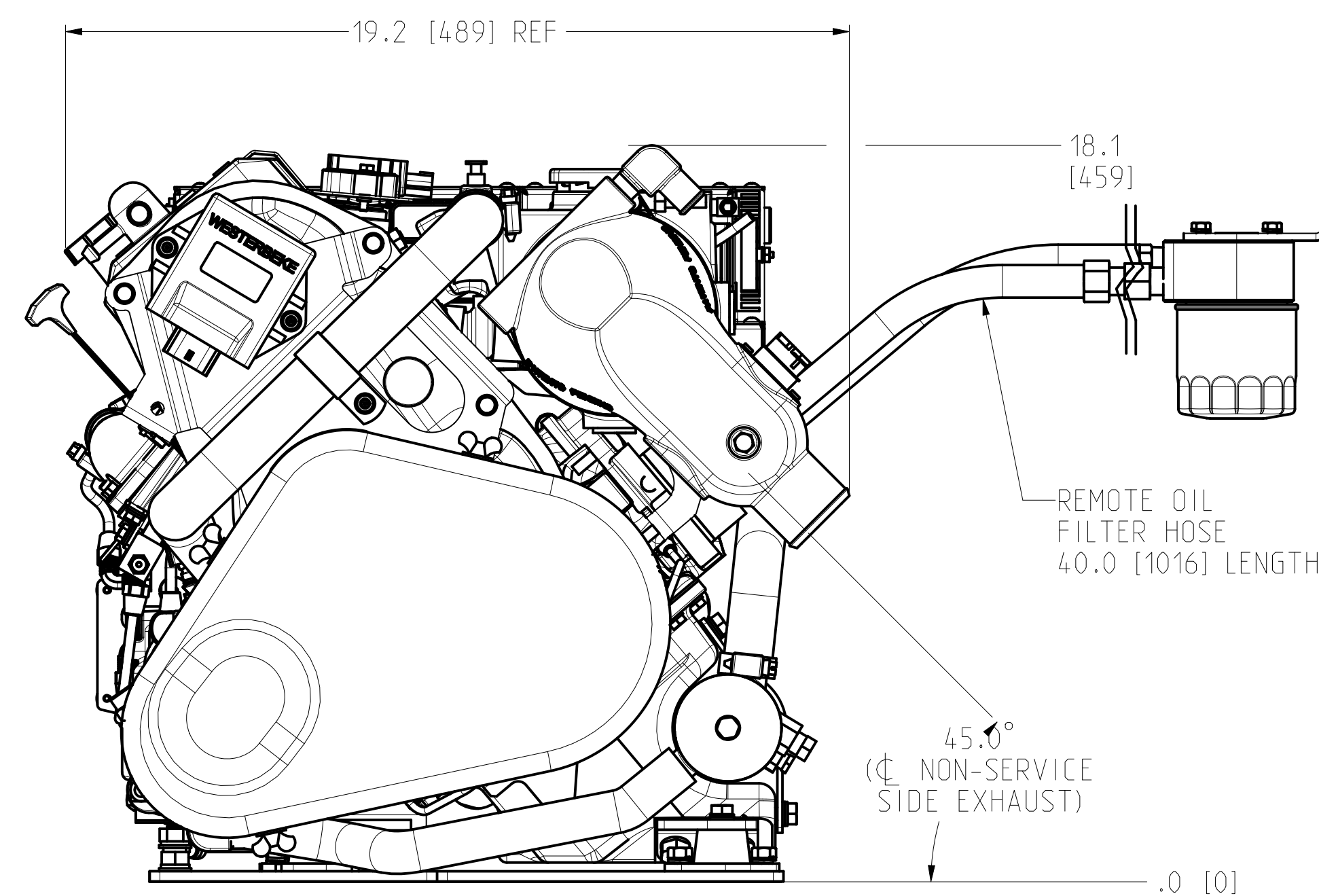
BELT END
